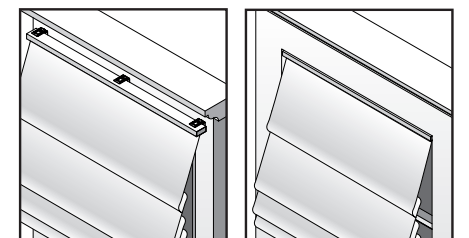
Outside Mount
