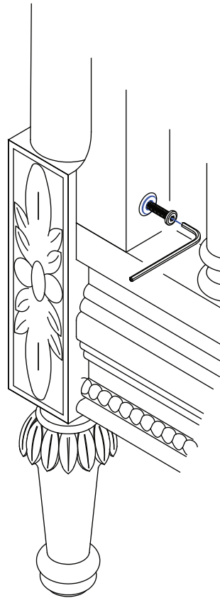
DETAIL H
