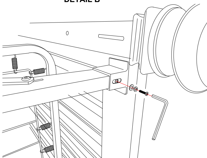
DETAIL B
