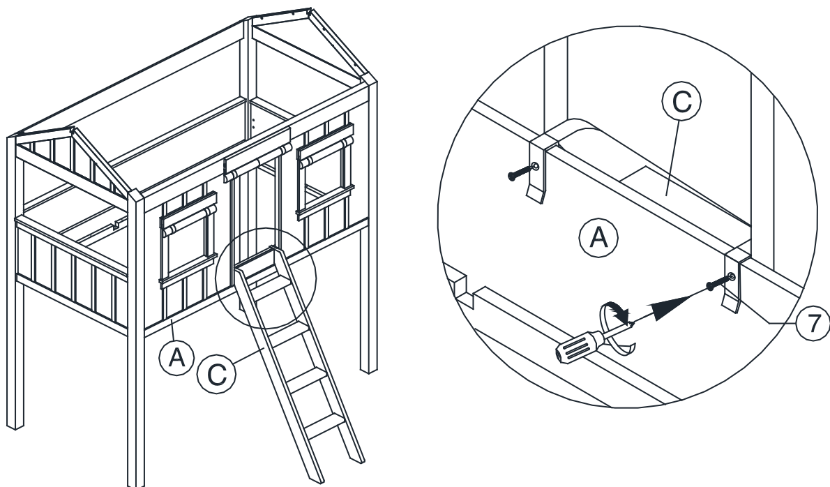
Detail "CC"
